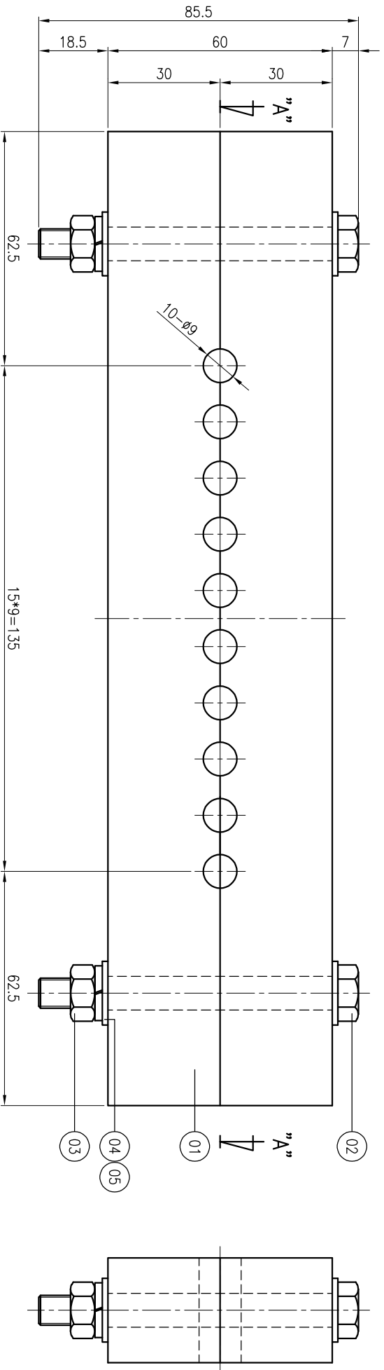
SECTION "A-A"
