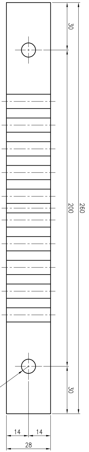
SECTION "A-A"
